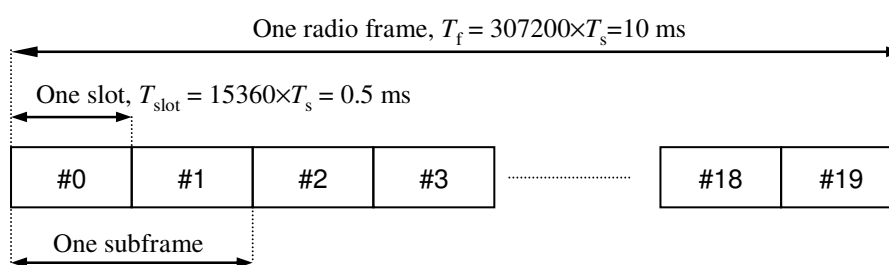
Figure 2: LTE Frame Structure (Type 1)
