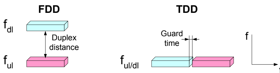
Figure 1: Time and Frequency Division Duplex
