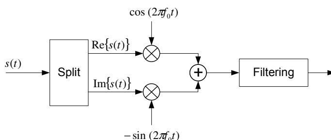
Figure 17: Up-conversion principles
