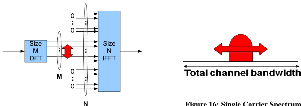
Figure 15: DFT Pre-distortion
